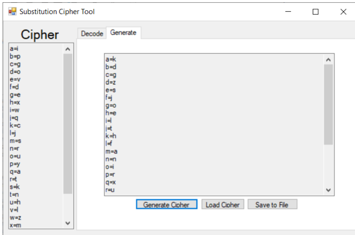
4: What the "Generate" tab should look like after clicking the "Generate Cipher" button.
